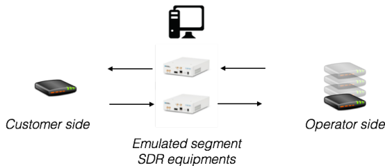
Fig. 2: An emulated bi-directional satellite access scheme. Modems and SDR devices are connected by means of coaxial cables.
